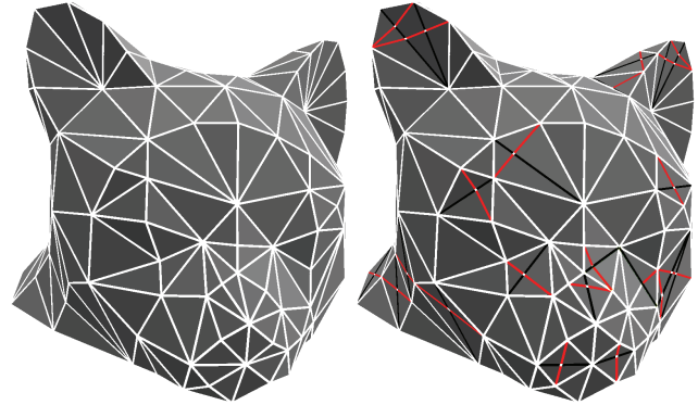
Figure 1: Left: carrier of the (cat head) surface as defined by the original embedded mesh. Right: the intrinsic Delaunay triangulation of the same carrier. Delaunay edges which appear in the original triangulation are shown in white. Some of the original edges are not present anymore (these are shown in black). In their stead we see red edges which appear as the result of intrinsic flipping. Note that the red edges are straight, i.e. , geodesic, within the original surface.
