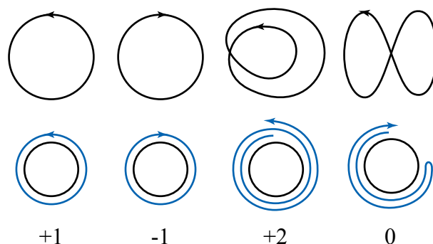
Figure 3: Turning numbers of various closed curves. Top row : Two simple curves with opposite sense of traversal, and two self-intersecting curves, one of which “undoes” the turn. Bottom row : Gaussian image of the curves, and the associated turning numbers.
