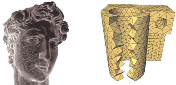
Figure 1: Typical 2D and 3D meshes: although the David' head appears smooth, its surface is made of a triangle mesh; tetrahedral meshes (such as this mechanical part, with a cutaway view) are some typical examples of irregular meshes on which computations are performed. David's head mesh is courtesy of Marc Levoy, Stanford.
