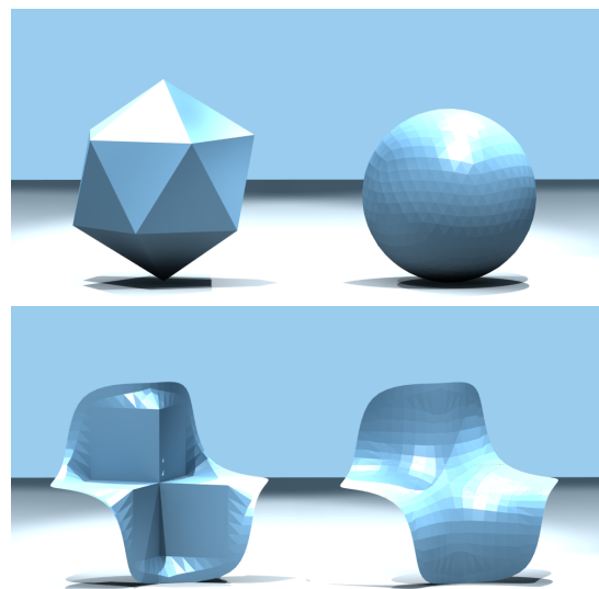
Figure 5: Initial and final frames of Willmore flow applied to solve two tasks posed by Bobenko and Schröder. (top) Smoothing a 4-times subdivided icosahedron into a sphere and (bottom) a hole filling problem. The sphere converged in 120ms (12ms \times 10 smoothing steps), with 200ms for Hessian prefactorization. The hole filling problem required 640ms after 120ms for prefactorization. Rendered with flat shading.
