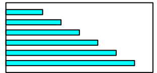
barchart[plot.polygon]
