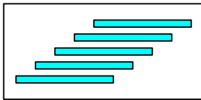
plot.shingle[plot.polygon]
