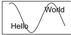
add.[line, text]
