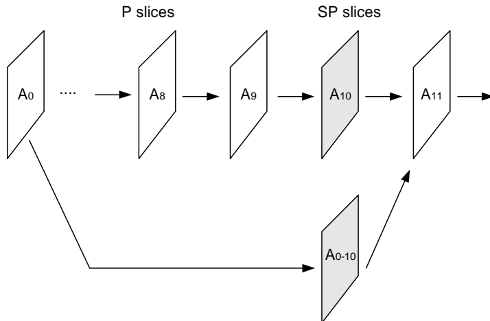
Figure 2-8 Fast-forward using SP-slices
